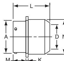
"SP" Potting Boot
