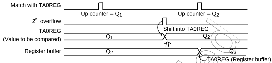
Figure 3.7.25 Register Buffer Operation
