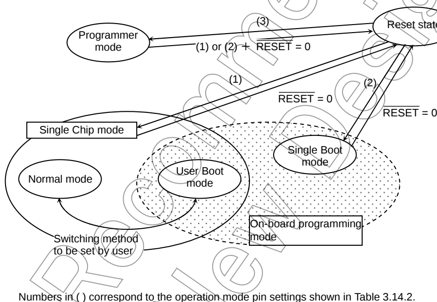
Figure 3.14.2 Mode Transition Diagram
