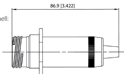
Backshell used with IEEE 1394 Receptacle with back-termination - (Type 1) Non sealed version Same panel drilling as FWFTV 2xx FWFTV 2PE & 7PE Type 1
