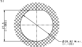
Panel Drilling
