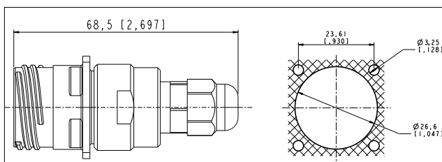
Backshell used with back termination type 2: Solder (Sealed - IP68)
