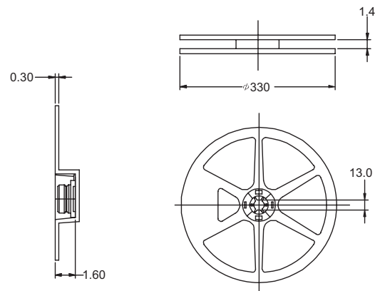
DIMENSIONS REEL (2500 PIECES/REEL)
