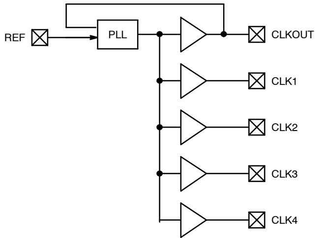
Figure 1. Block Diagram
