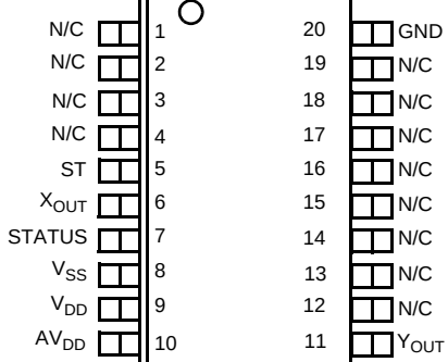
Figure 2. Pin Connections
