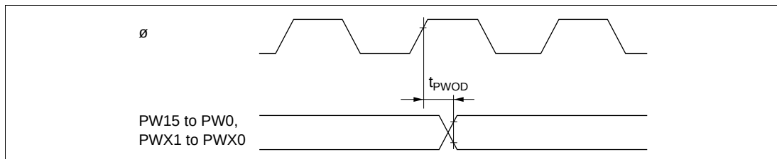
Figure 25.21 PWM, PWMX Output Timing
