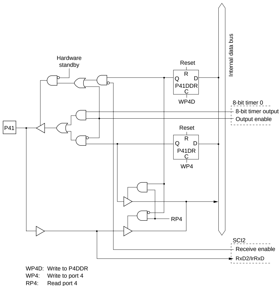
Figure C.7 Port 4 Block Diagram (Pin P41)
