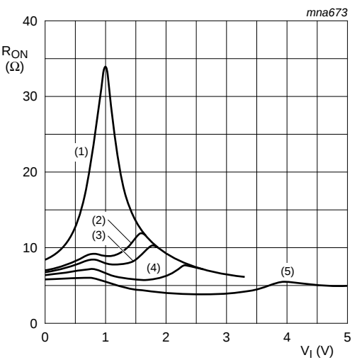
Fig 9. Typical ON resistance as a function of input voltage; T_{amb} = 25\text{ }^{\circ}\text{C}
