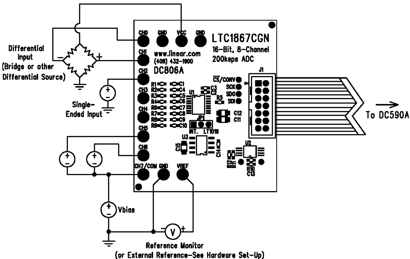
Figure 1. Connection Diagram
