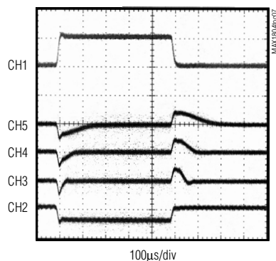
LOAD TRANSIENT RESPONSE (APPLICATION CIRCUIT OF FIGURE 2)
