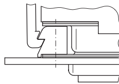
Front mounted connector with FRH1/5 and F-GK1/5
