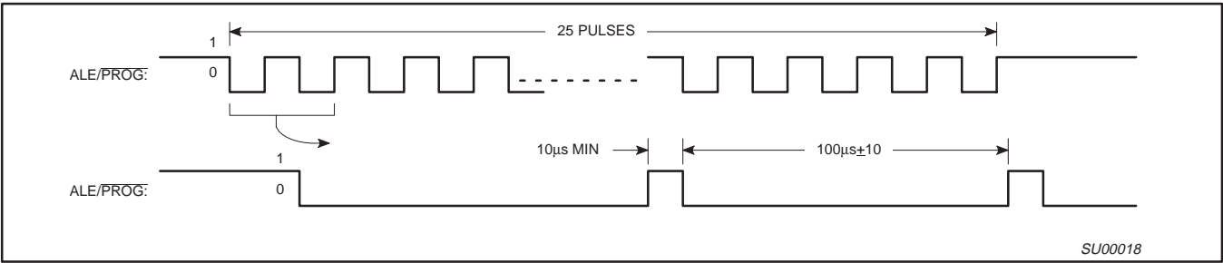
Figure 18. PROG Waveform
