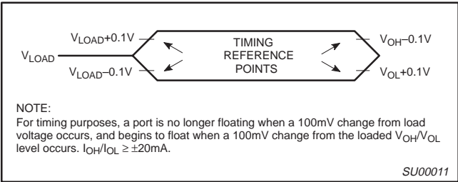
Figure 11. Float Waveform
