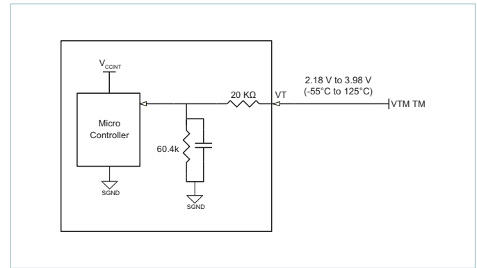
Figure 30 — VT Connections
