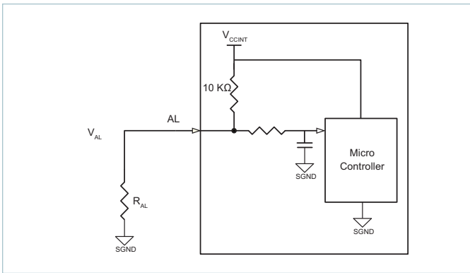
Figure 29 — AL Connections
