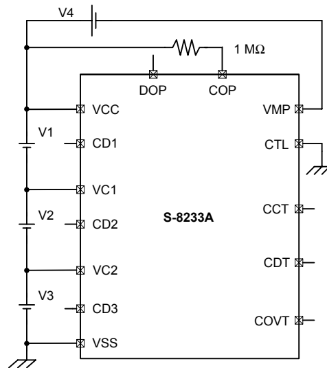
Measurement circuit 2
