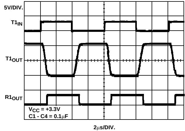
FIGURE 14. LOOPBACK TEST AT 250kbps
