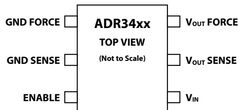
Figure 1. 6-Lead SOT23
