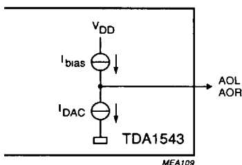
(c) output pins AOL and AOR.
