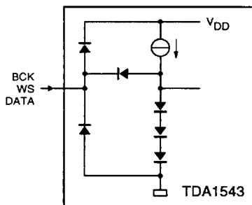
(a) input pins BCK, WS and DATA.
