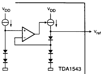
(b) output pin V ref .
