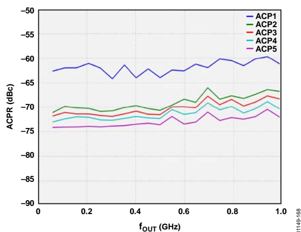
Figure 51. Four-Carrier ACPR vs. f_{OUT}
