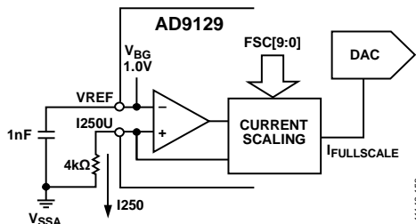
Figure 149. Voltage Reference Circuit
