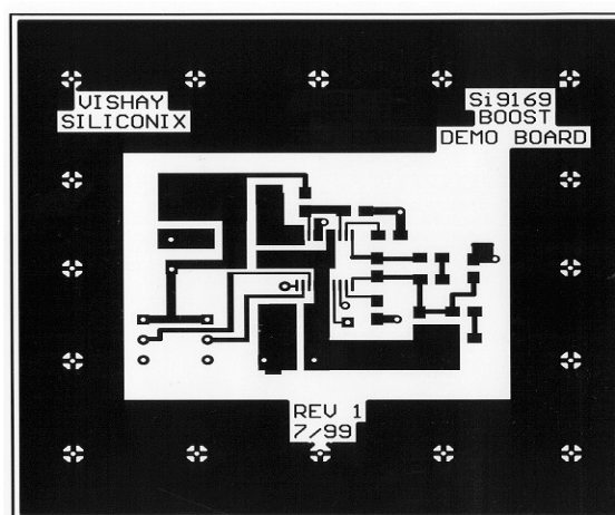
FIGURE 11. Boost—Top Layer
