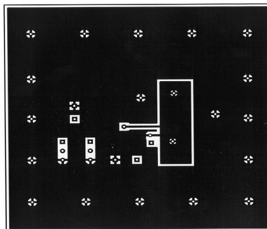
FIGURE 12. Boost—Bottom Layer
