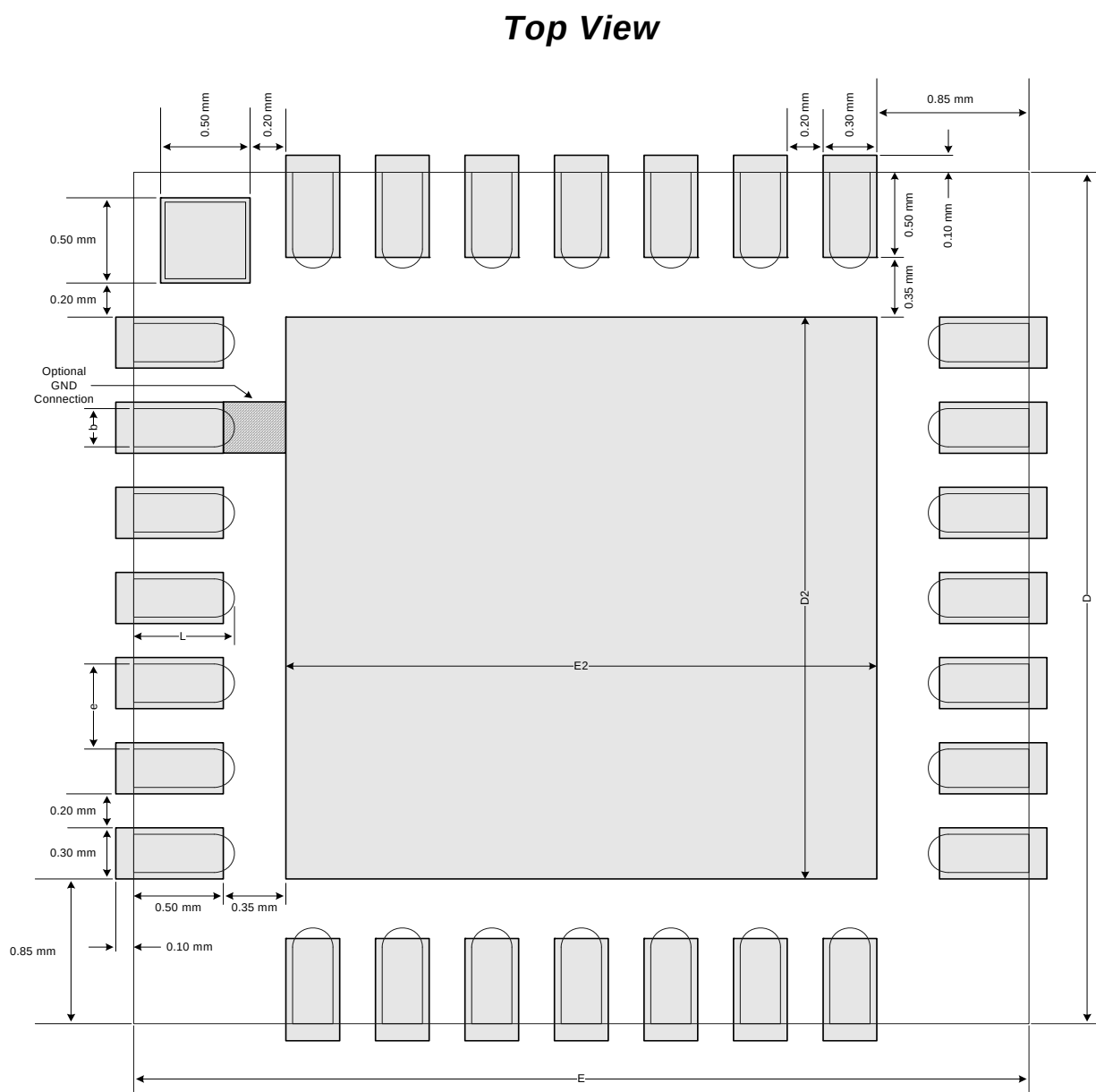
Figure 8. Typical QFN-28 Landing Diagram
