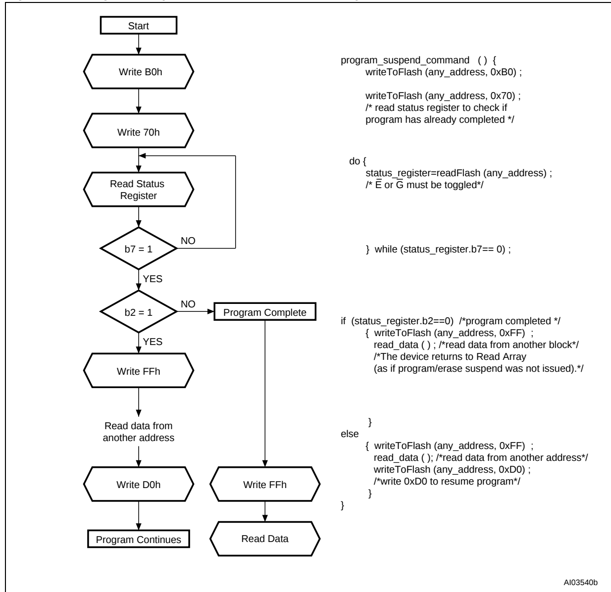
Figure 18. Program Suspend &amp; Resume flowchart and pseudocode
