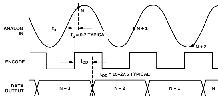
AD9022 Timing Diagram
