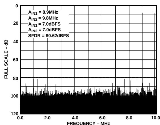
Figure 10. Two-Tone FFT
