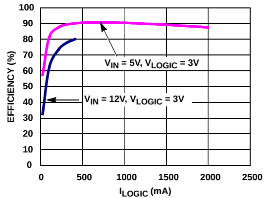
FIGURE 4. BUCK V_{\text{LOGIC}} EFFICIENCY
