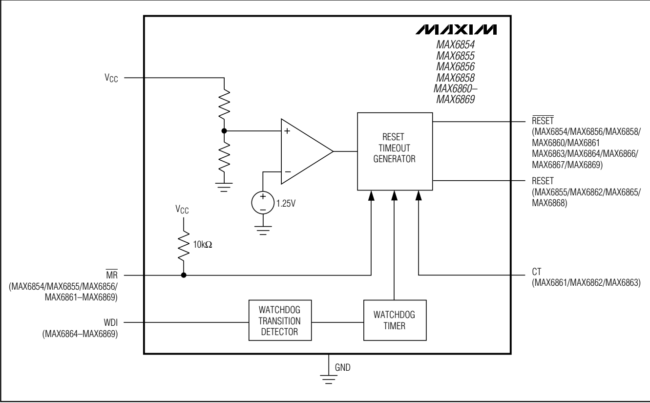
Figure 1. Functional Diagram
