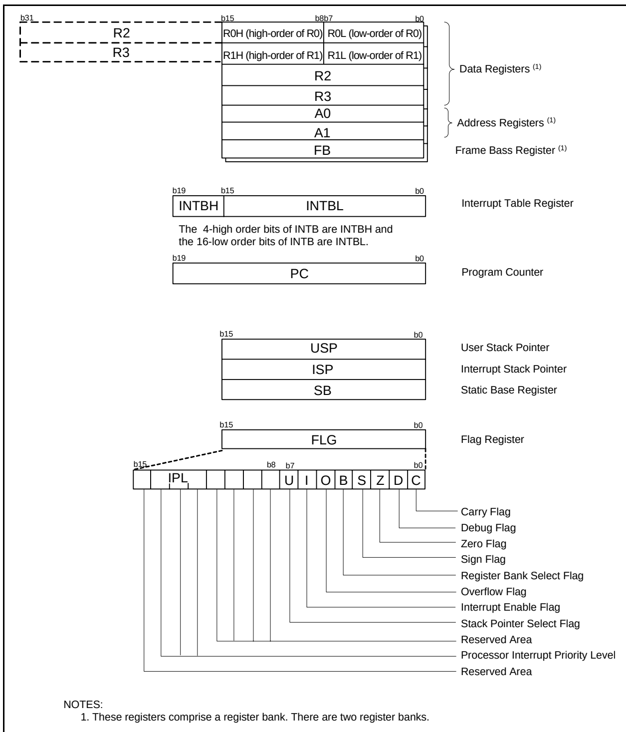
Figure 2.1 CPU Register
