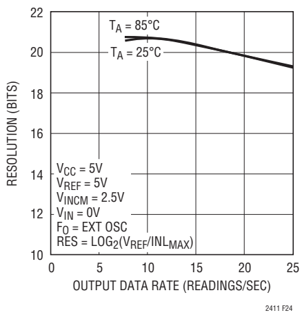
Figure 24. Resolution ( \text{INL}_{RMS} \leq 1\text{LSB} ) vs Output Data Rate and Temperature
