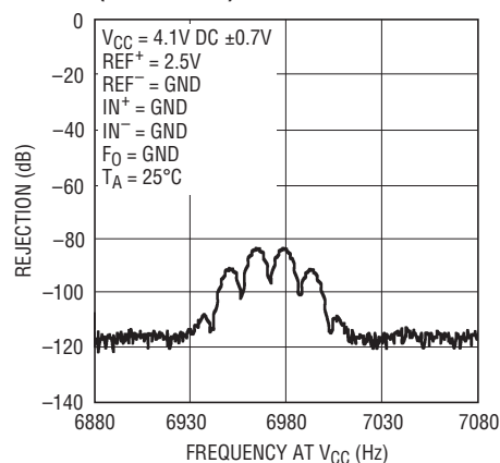
PSRR vs Frequency at V_{CC} (LTC2411-1)
