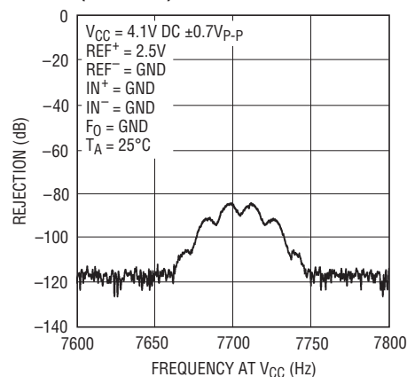
PSRR vs Frequency at V_{CC} (LTC2411)
