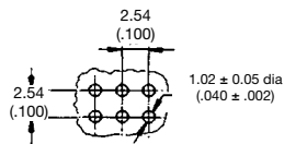
Recommended PCB layouts
