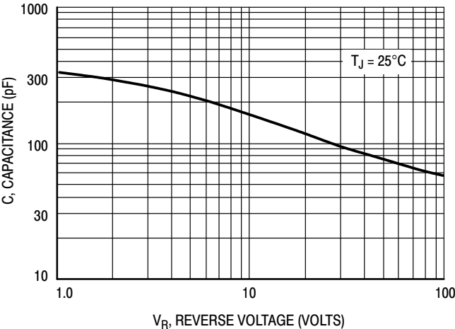
Figure 10. Typical Capacitance
