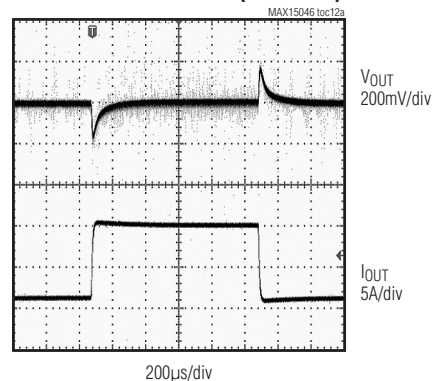
LOAD TRANSIENT ON OUT (1A TO 10A)
