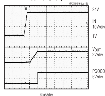
STARTUP WITH PREBIASED OUTPUT (1.0V)
