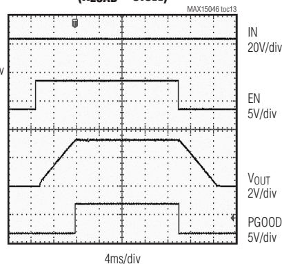
STARTUP DISABLE FROM EN ( R_{LOAD} = 3.3\Omega )
