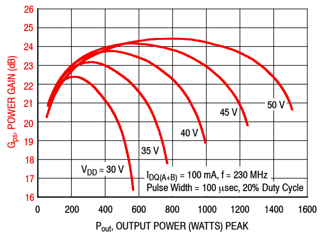
Figure 10. Power Gain versus Output Power and Drain-Source Voltage
