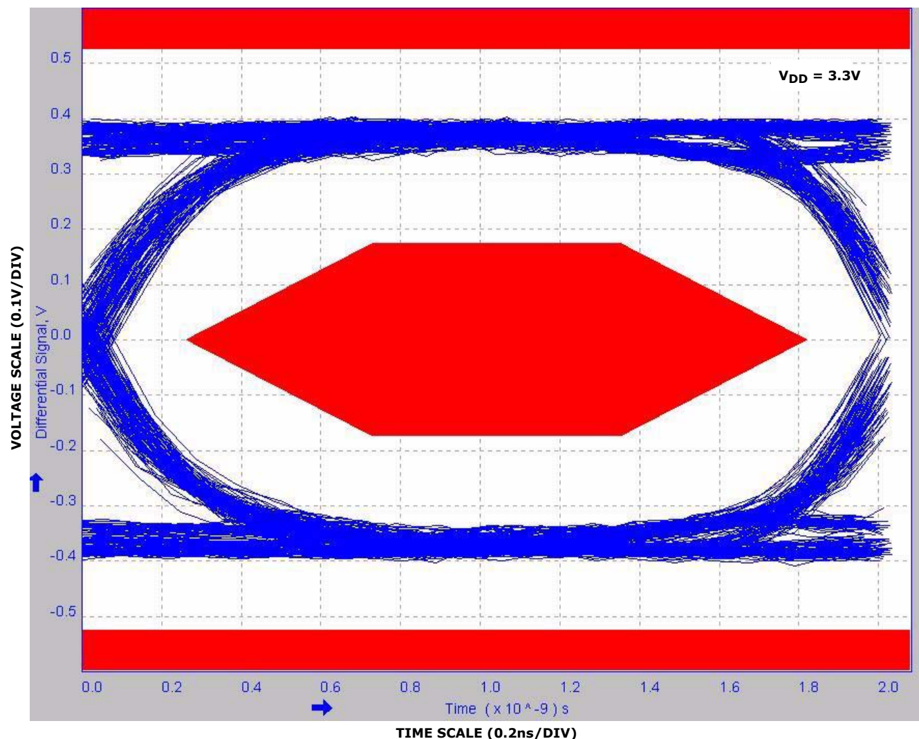
FIGURE 9. EYE PATTERN WITH FAR END MASK: 480MBPS USB SIGNAL WITH HSx SWITCHES IN THE SIGNAL PATH
