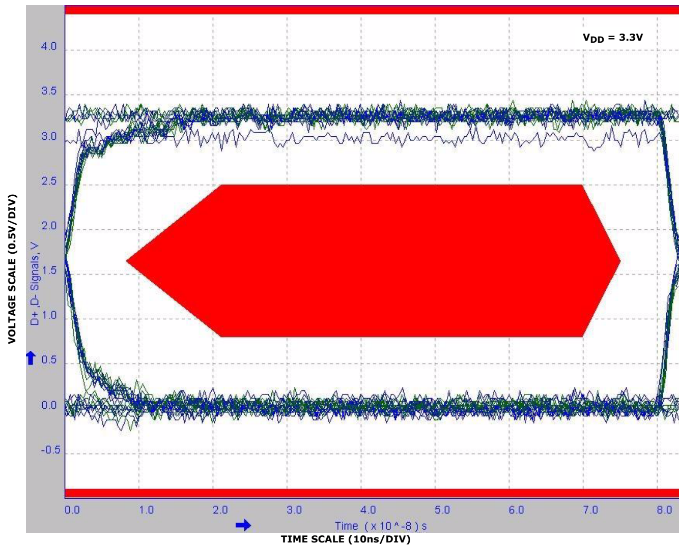
FIGURE 11. EYE PATTERN: 12MBPS USB SIGNAL WITH HSx SWITCHES IN THE SIGNAL PATH
