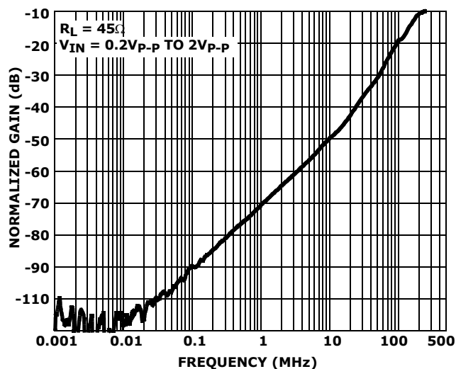
FIGURE 14. CROSSTALK
