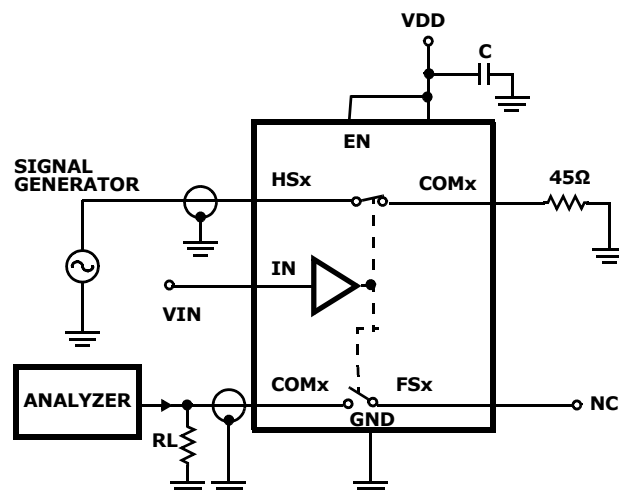
FIGURE 6. CROSSTALK TEST CIRCUIT
