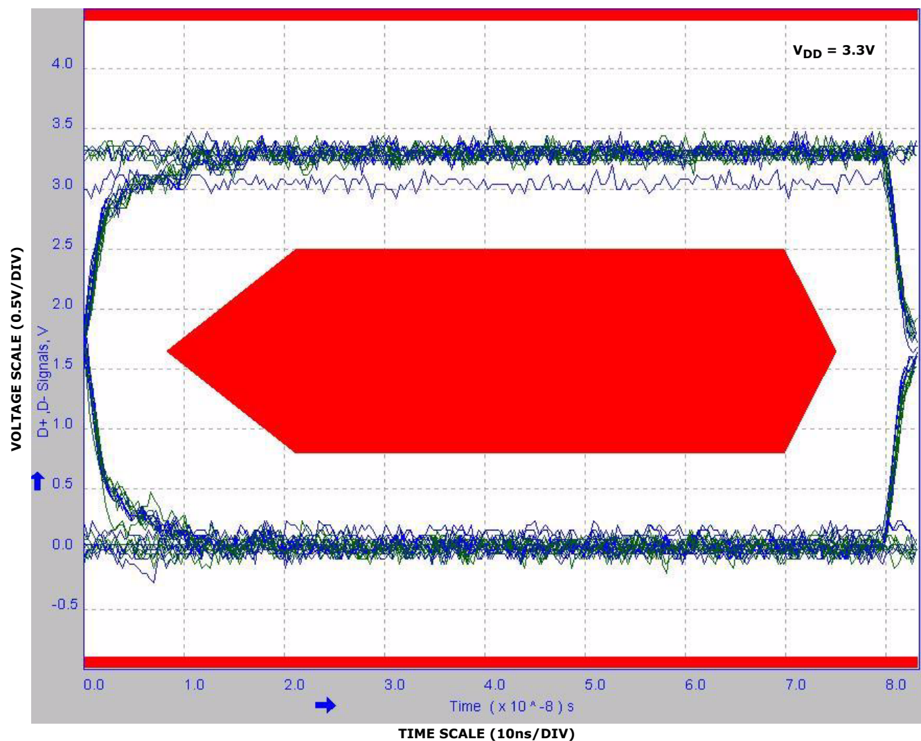
FIGURE 8. EYE PATTERN: 12MBPS USB SIGNAL WITH FSx SWITCHES IN THE SIGNAL PATH
