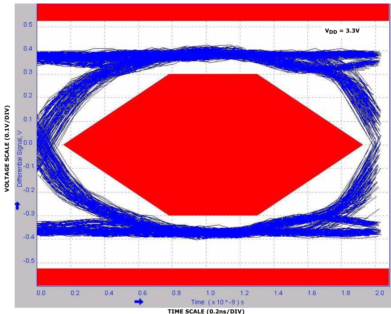
FIGURE 10. EYE PATTERN WITH NEAR END MASK: 480MBPS USB SIGNAL WITH HSx SWITCHES IN THE SIGNAL PATH
