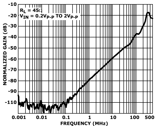
FIGURE 13. OFF-ISOLATION
