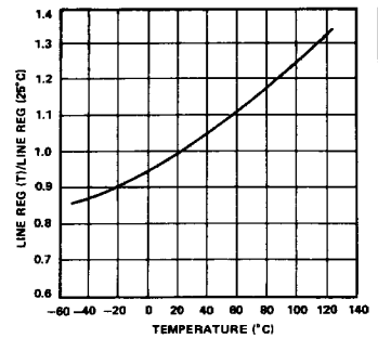
NORMALIZED LINE REGULATION vs TEMPERATURE
