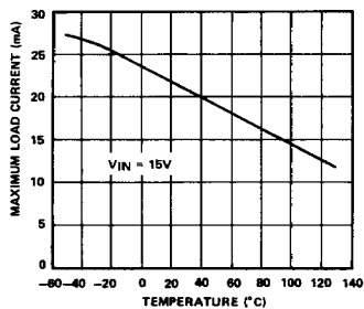
MAXIMUM LOAD CURRENT vs TEMPERATURE
