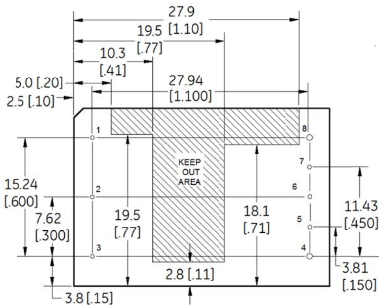
Through-Hole Pad Layout
