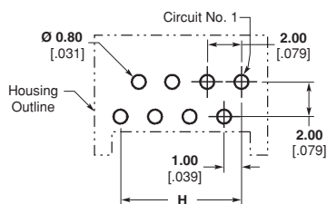
Recommended PCB Layout 1.60 [.063] Thickness (For Even Position Connectors)
