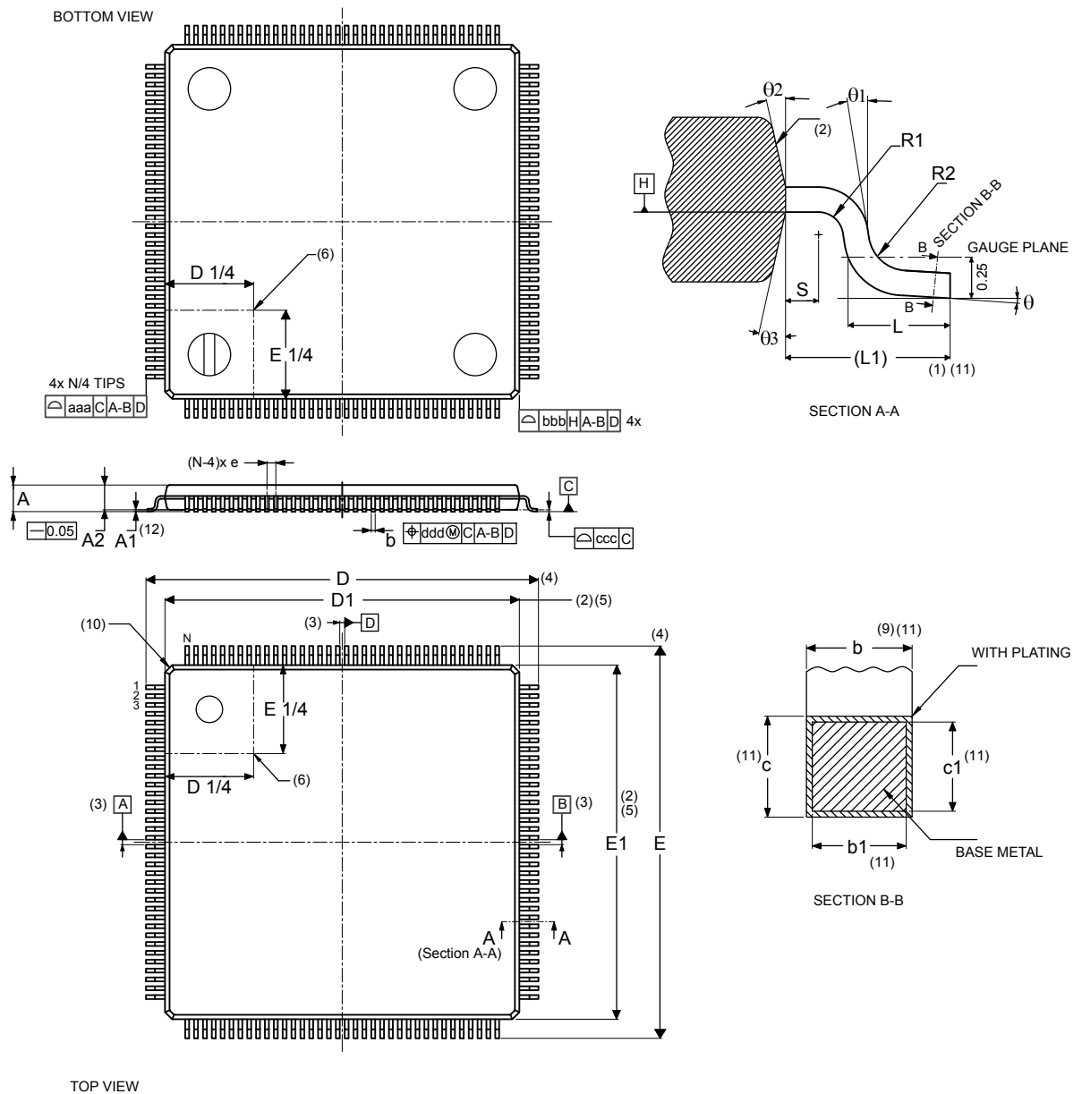
Figure 94. LQFP144 - Outline (15)
