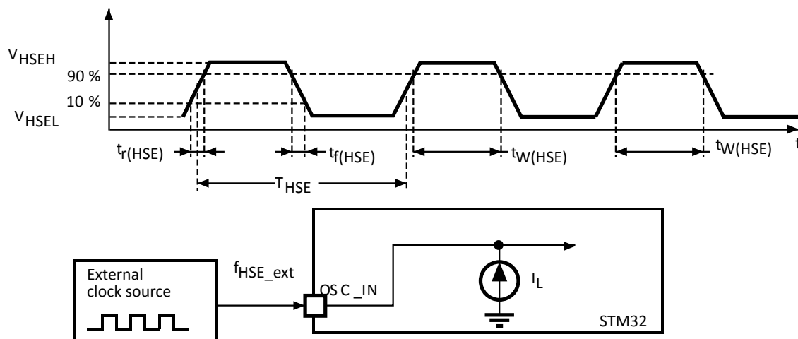
Figure 30. High-speed external clock source AC timing diagram
