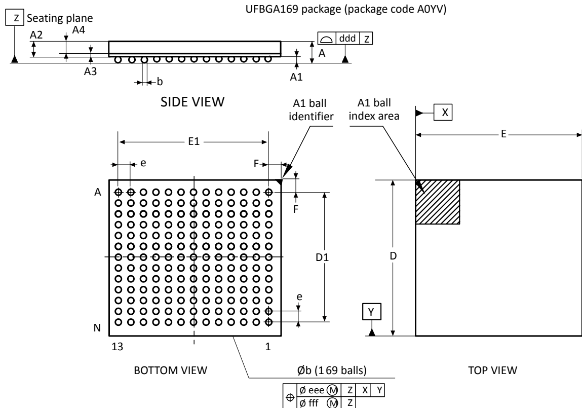
Figure 106. UFBGA169 - Outline
