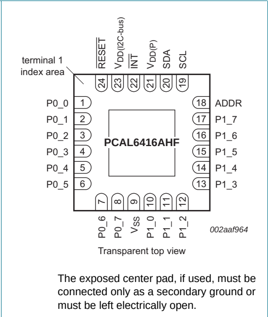
Fig 3. Pin configuration for HWQFN24
