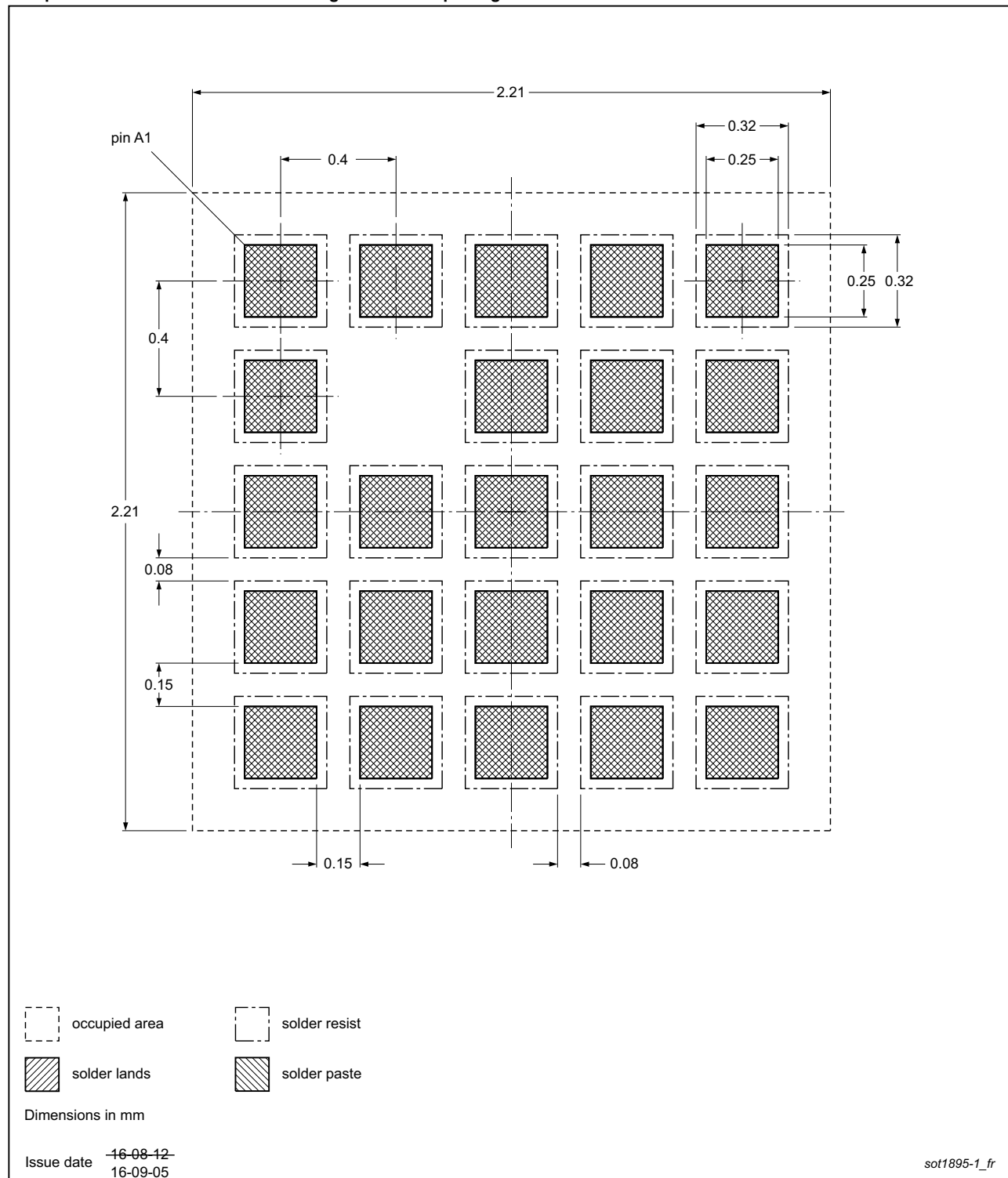
Fig 54. PCB footprint for SOT1895-1 (X2QFN24); reflow soldering
