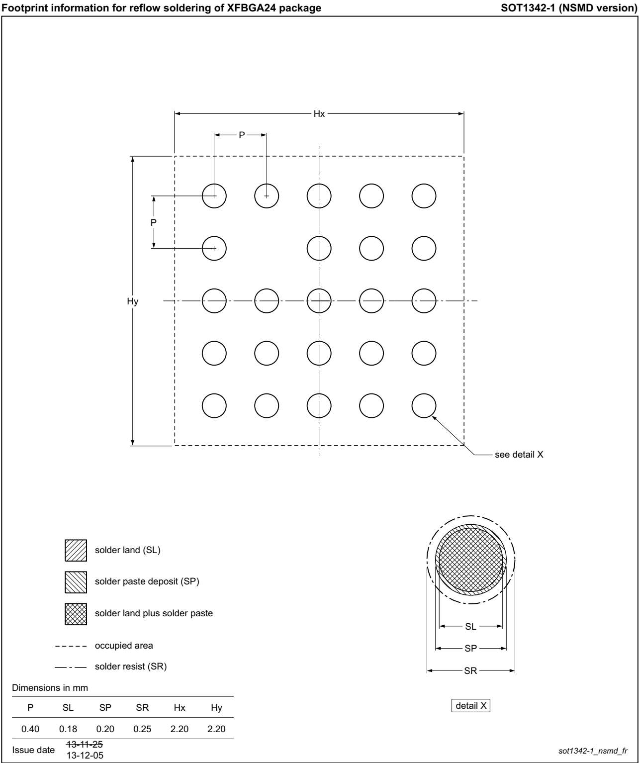
Fig 51. PCB footprint for SOT1342-1 (XFBGA24, Non-Solder Mask Defined version), EX option; reflow soldering
