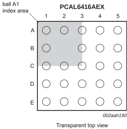
Fig 6. Pin configuration for XFBGA24 (2 mm × 2 mm); EX option
