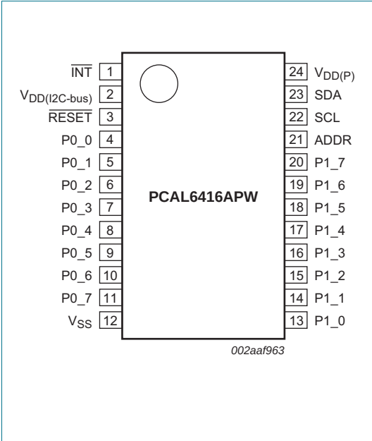
Fig 2. Pin configuration for TSSOP24
