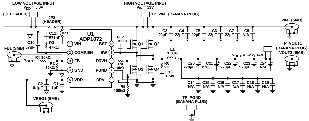
Figure 29. 1.8 V Output, 300 kHz, 14 A Application Circuit
