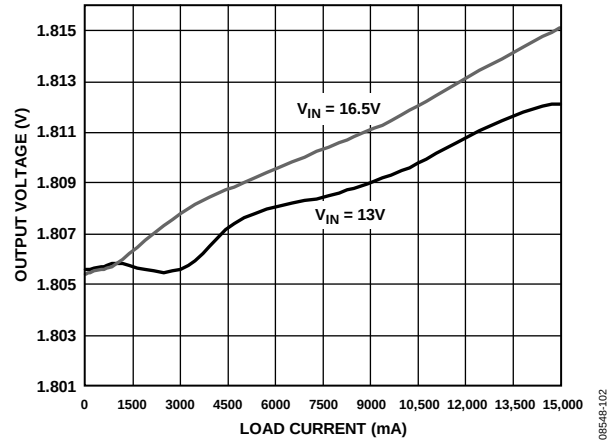
Figure 6. Load Regulation Plot for f_{SW} = 300 kHz, V_{OUT} = 1.8 V
