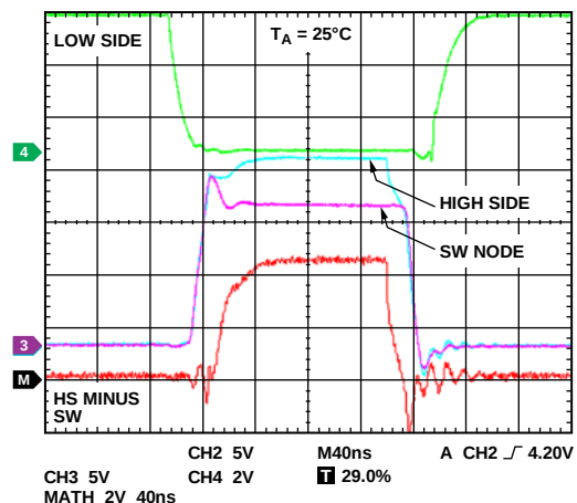
Figure 24. Output Drivers and SW Node Waveforms
