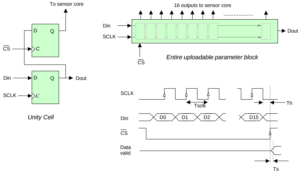
Figure 12. SPI Interface
