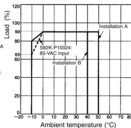
100-W Models with PFC Parallel-Unit Operation
