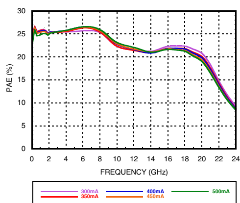
PAE @ Psat vs. Idq
