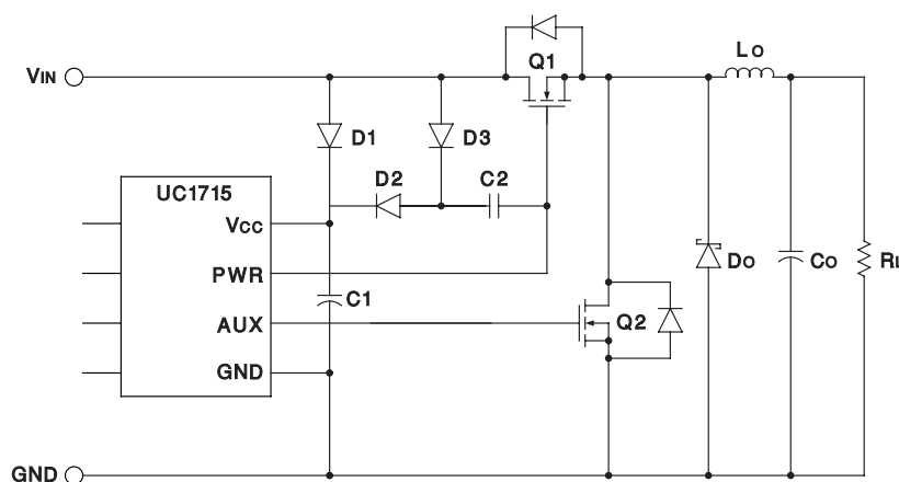
Figure 11. Synchronous Rectifier Application With A Charge Pump To Drive The High-Side N-Channel Buck Switch
