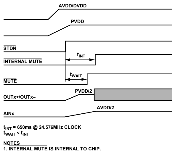
Figure 47. Power-Up Sequence, t_{WAIT} < t_{INT}
