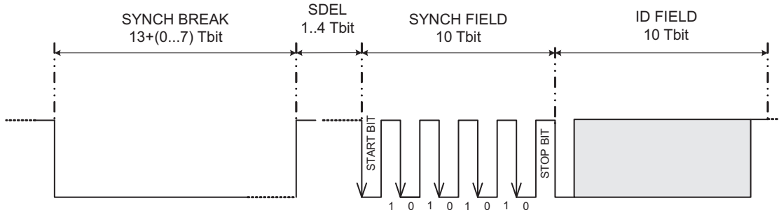
Figure 26-15. Message Header in Terms of T_{bit}
