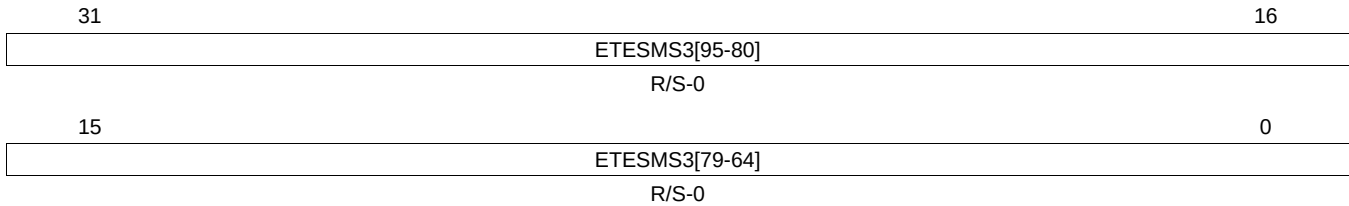
Figure 23-75. Enable Transfer on Event to System Memory Set 3 (ETESMS3) [offset_TU = D0h]
