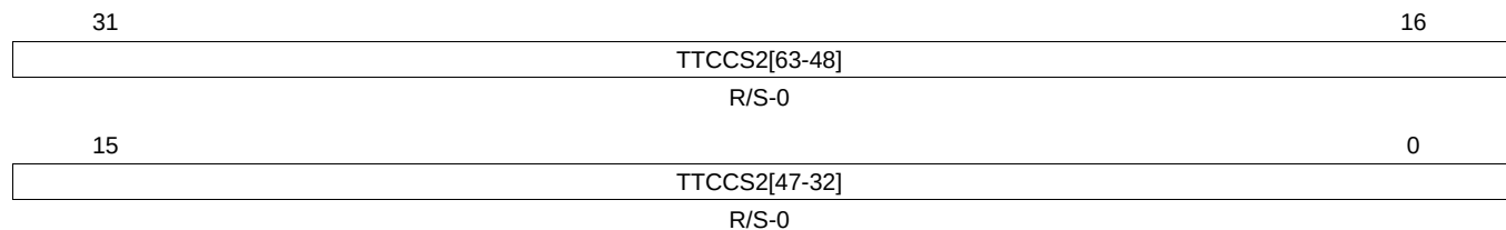
Figure 23-65. Trigger Transfer to Communication Controller Set 2 (TTCCS2) [offset_TU = A8h]
