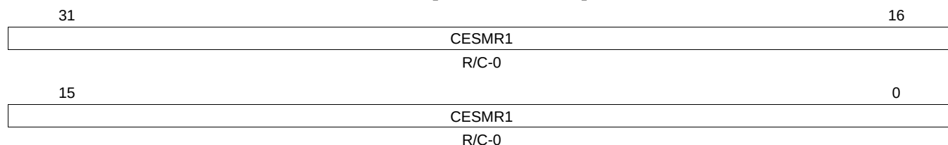
Figure 23-80. Clear on Event to System Memory Reset 1 (CESMR1) [offset_TU = E4h]
