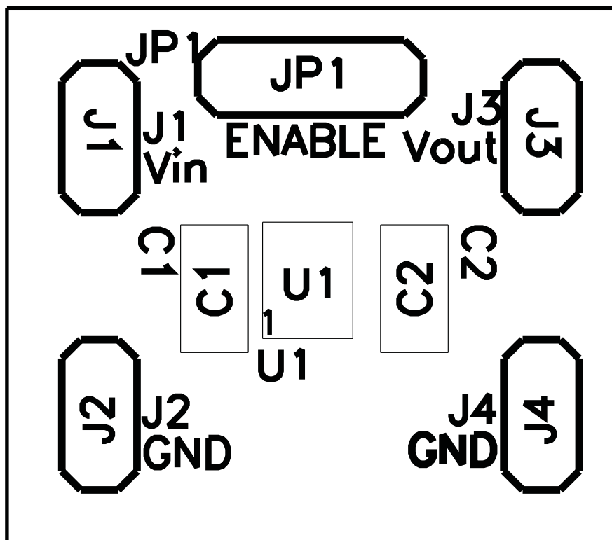
Figure 1. Assembly Layer
