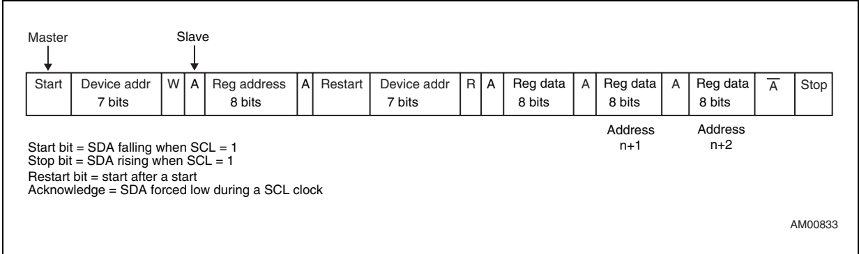
Figure 8. Read operation
