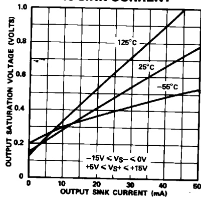
SATURATION VOLTAGE vs SINK CURRENT
