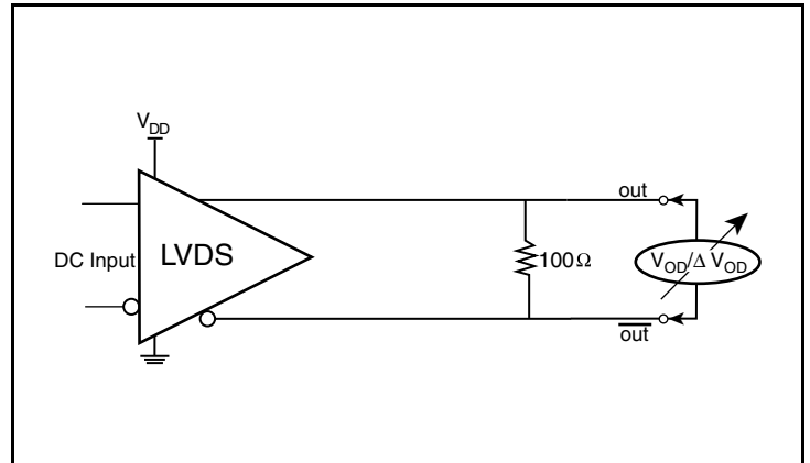
Differential Output Voltage
