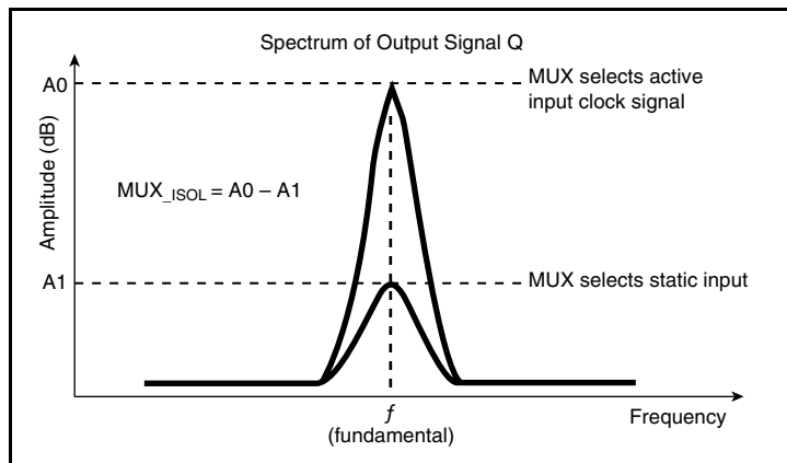
MUX Isolation
