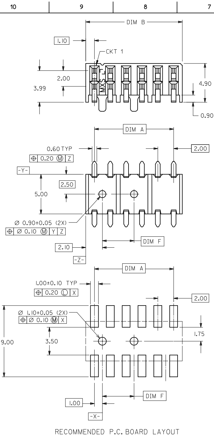
RECOMMENDED P.C. BOARD LAYOUT
