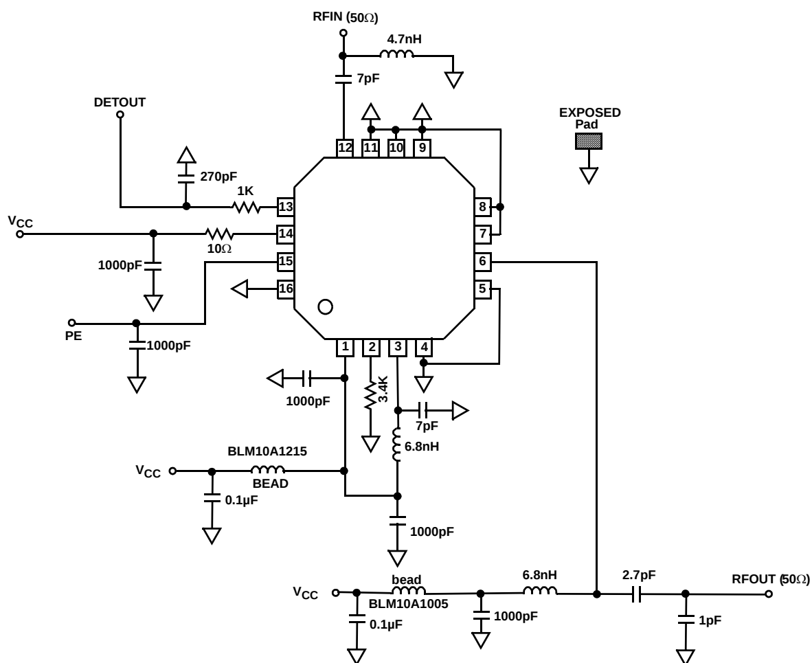
ISL3985 - 16 PIN QFN PACKAGE
