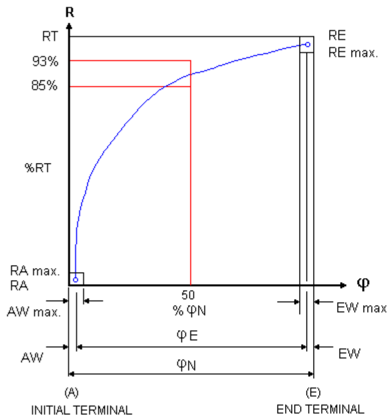
Resistance law C (Reverse Audio/Anti Log) curve
